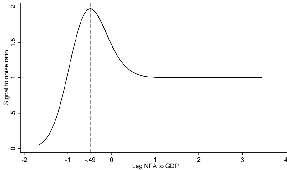
Figure 5. Univariate Model: Threshold for NFA/GDP that Maximizes Signal to Noise
